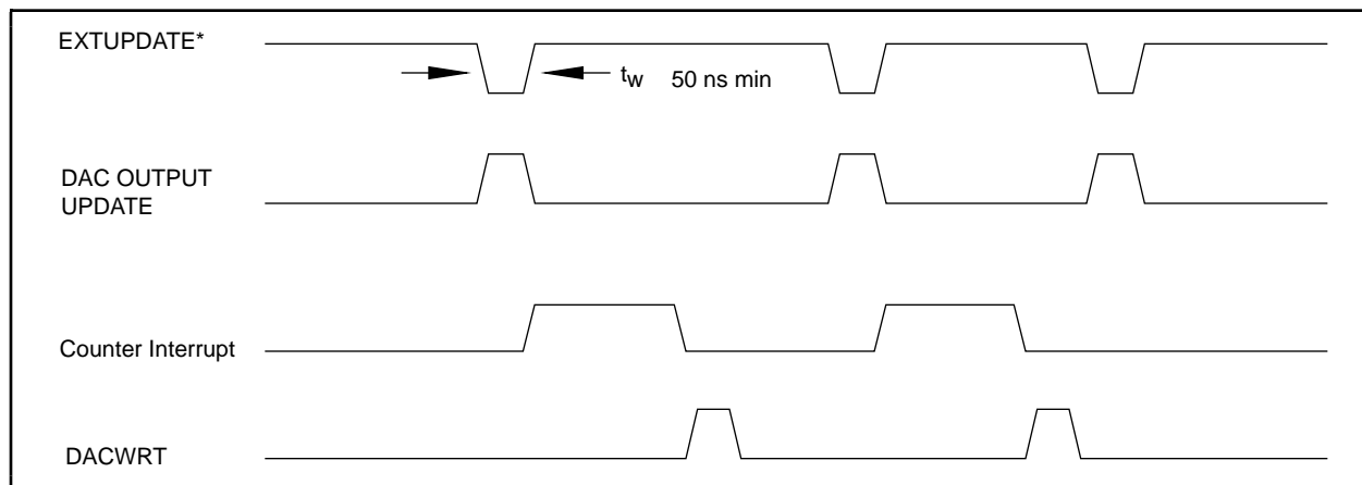
Figure 3-16. EXTUPDATE* Signal Timing for Updating DAC Output
