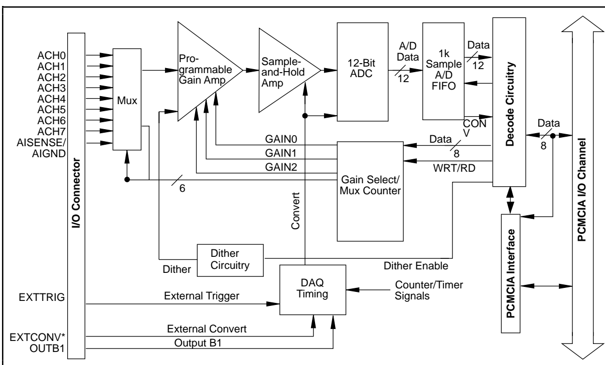
Figure 4-4. Analog Input Circuitry
