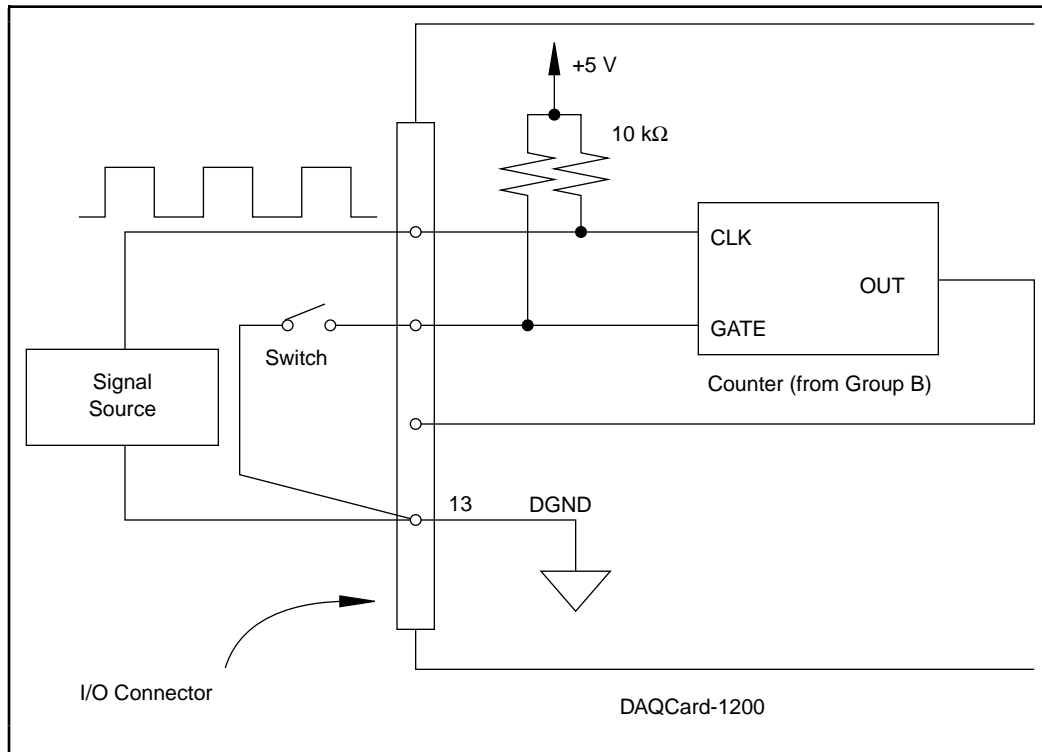
Figure 3-17. Event-Counting Application with External Switch Gating
