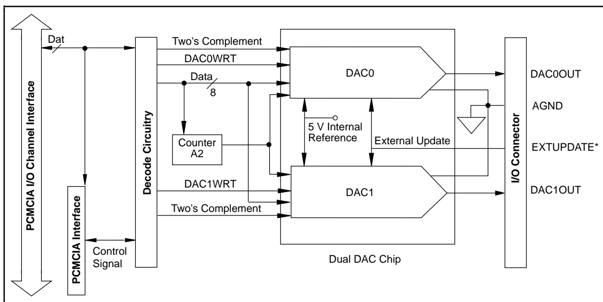
Figure 4-5. Analog Output Circuitry
