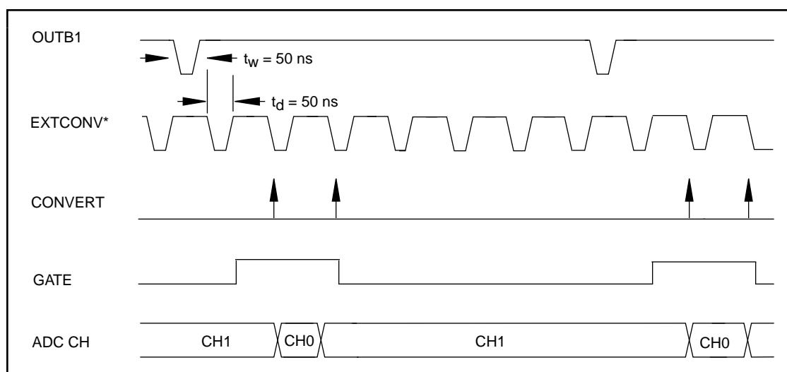
Figure 3-15. Interval-Scanning Signal Timing
