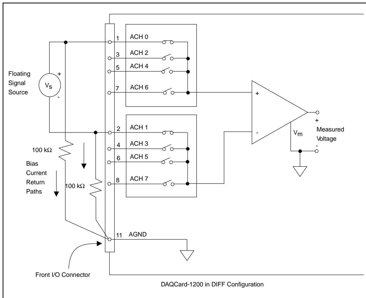
Figure 3-4. Differential Input Connections for Floating Sources
