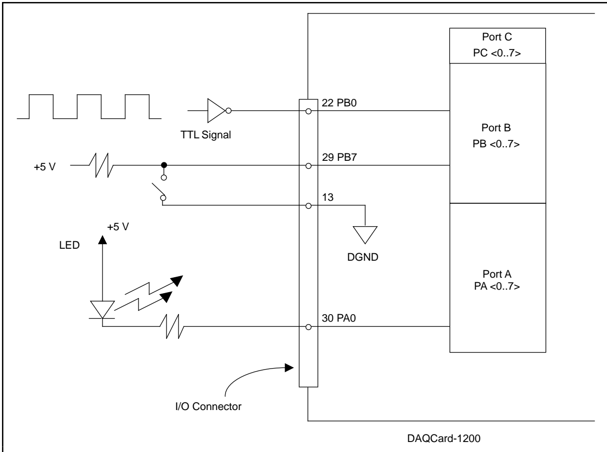
Figure 3-8. Digital I/O Connections
