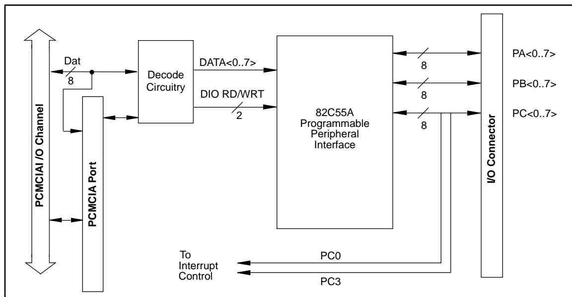
Figure 4-6. Digital I/O Circuitry
