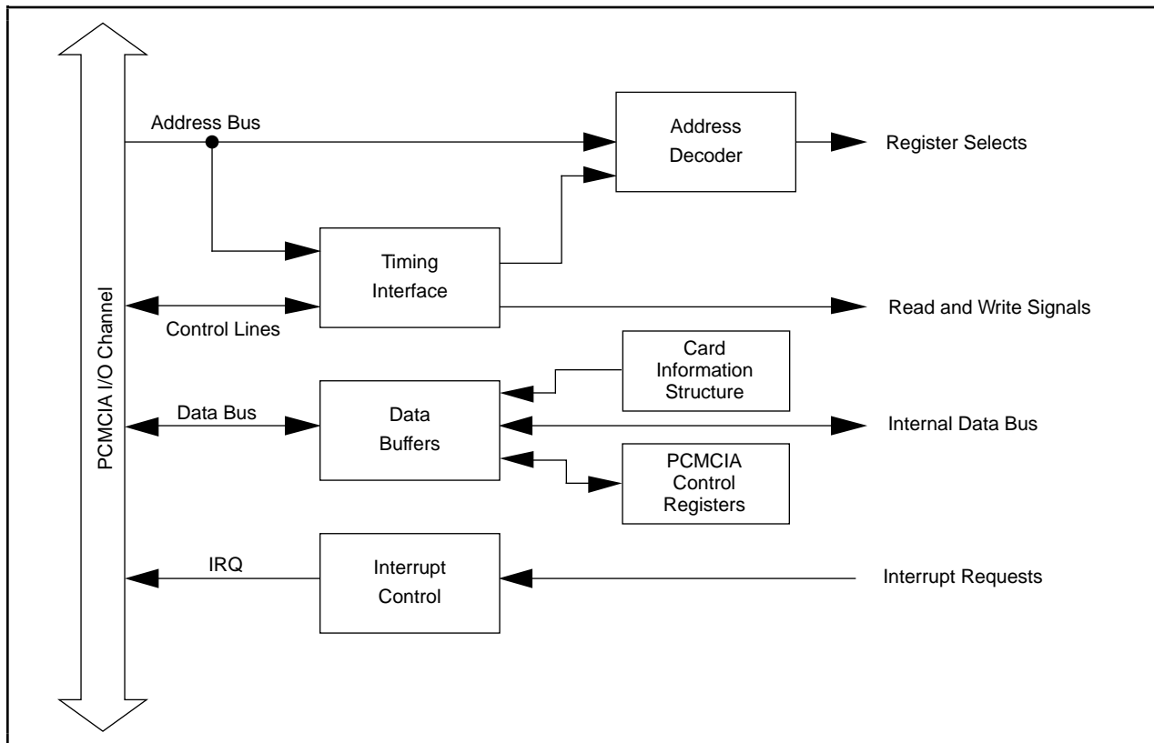
Figure 4-2. PC Card I/O Interface Circuitry Block Diagram
