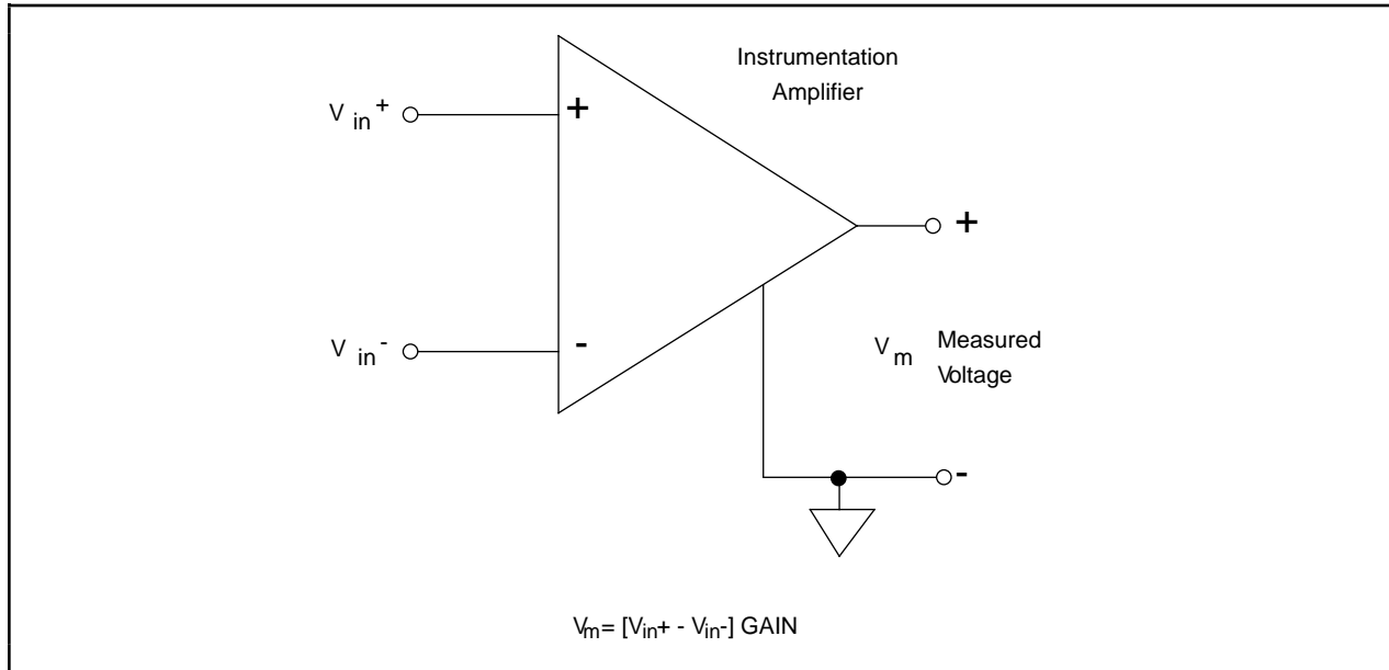
Figure 3-2. DAQCard-1200 Instrumentation Amplifier
