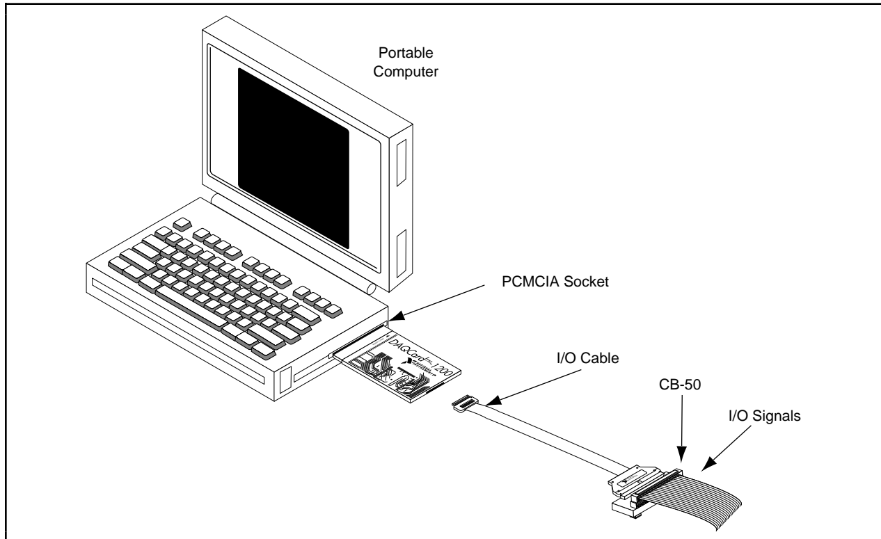
Figure 2-1. A Typical Configuration for the DAQCard-1200
