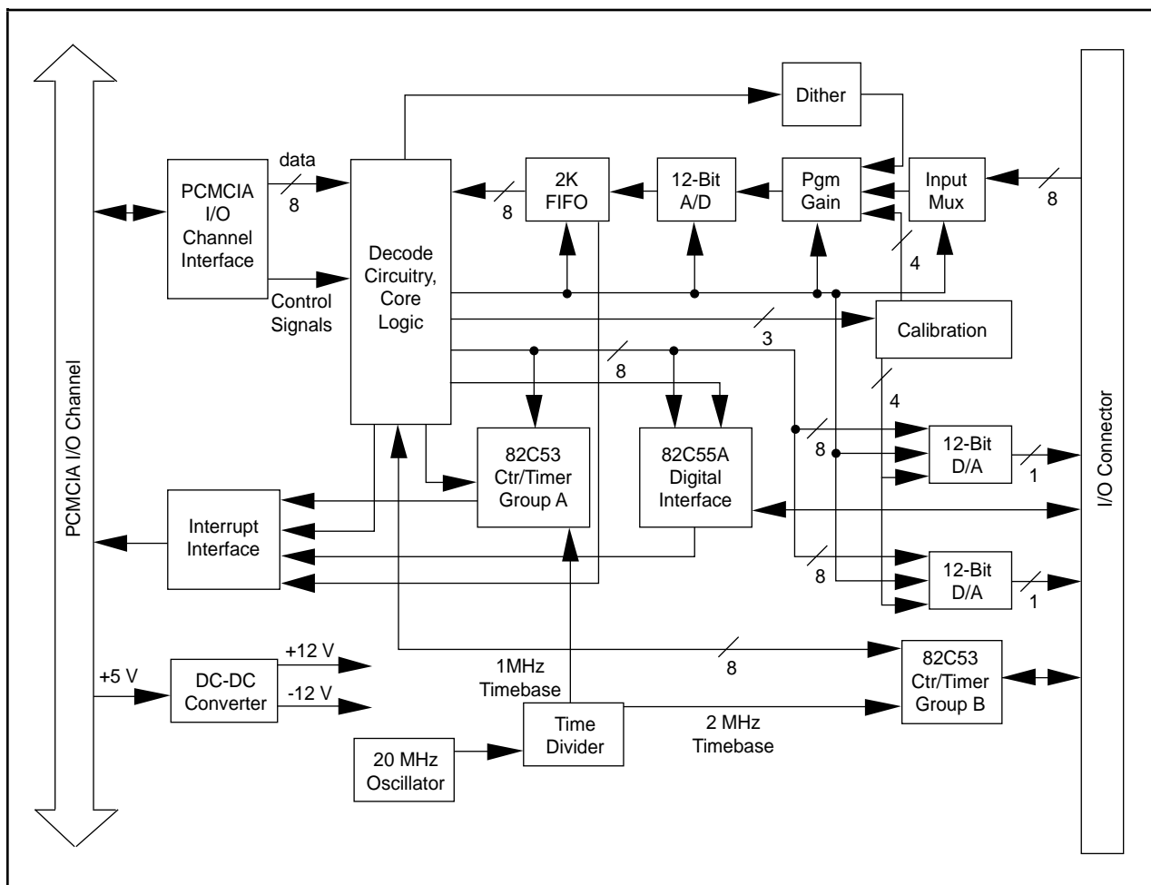
Figure 4-1. DAQCard-1200 Block Diagram
