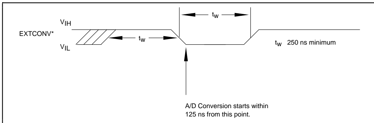
Figure 3-12. EXTCONV* Signal Timing
