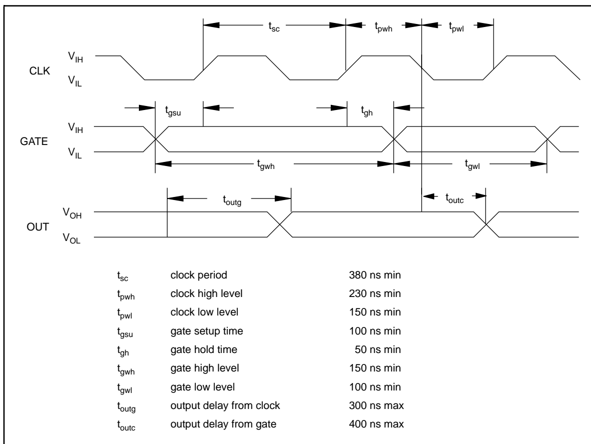
Figure 3-19. General-Purpose Timing Signals
