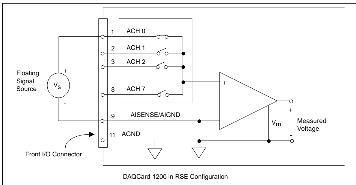
Figure 3-5. Single-Ended Input Connections for Floating Signal Sources
