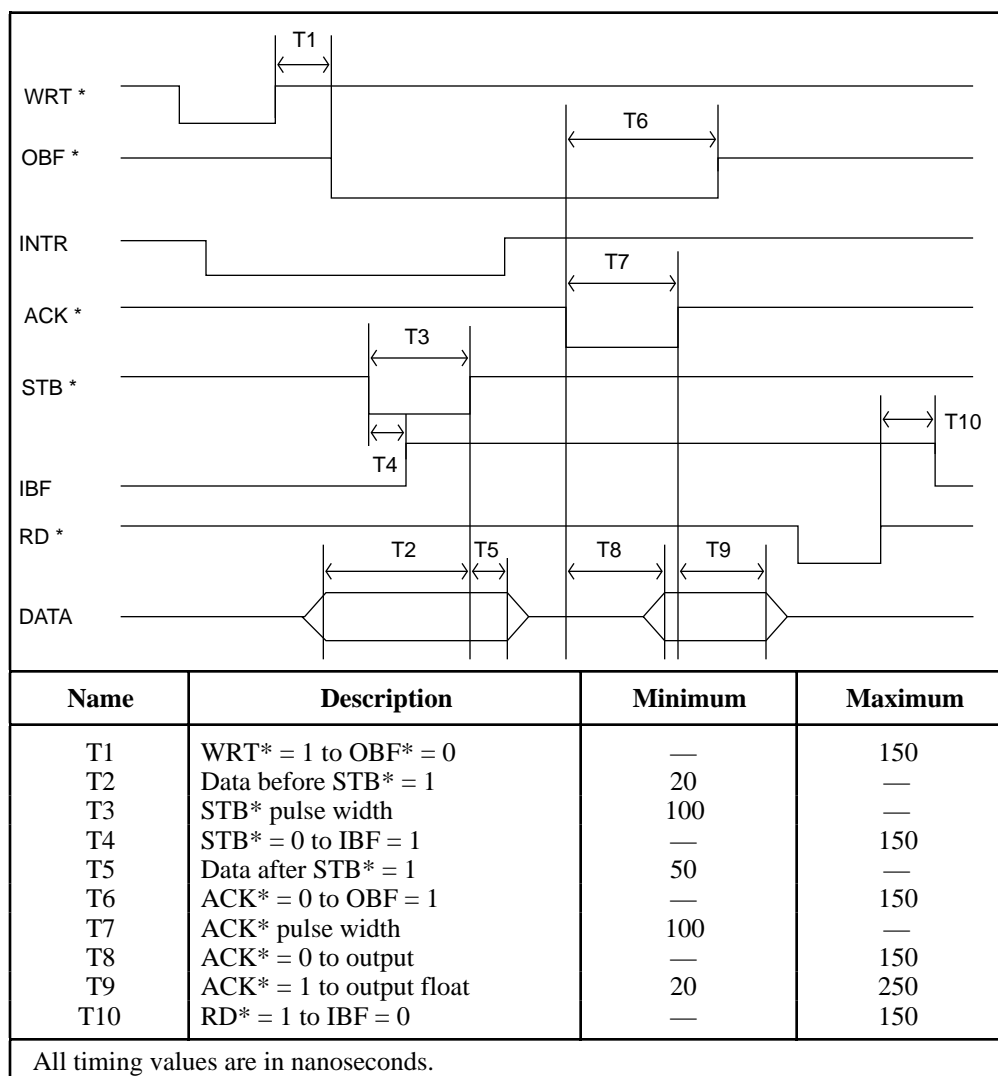
Figure 3-11. Mode 2 Timing Specifications for Bidirectional Transfers
