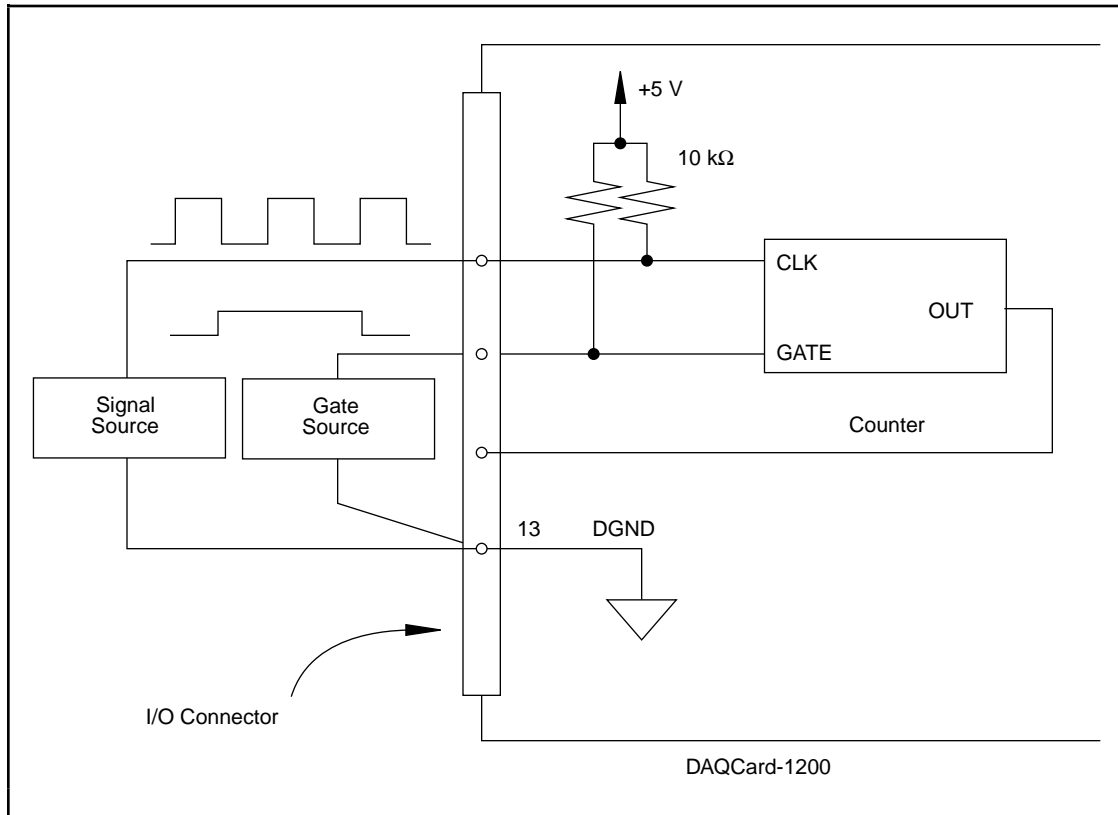
Figure 3-18. Frequency Measurement Application
