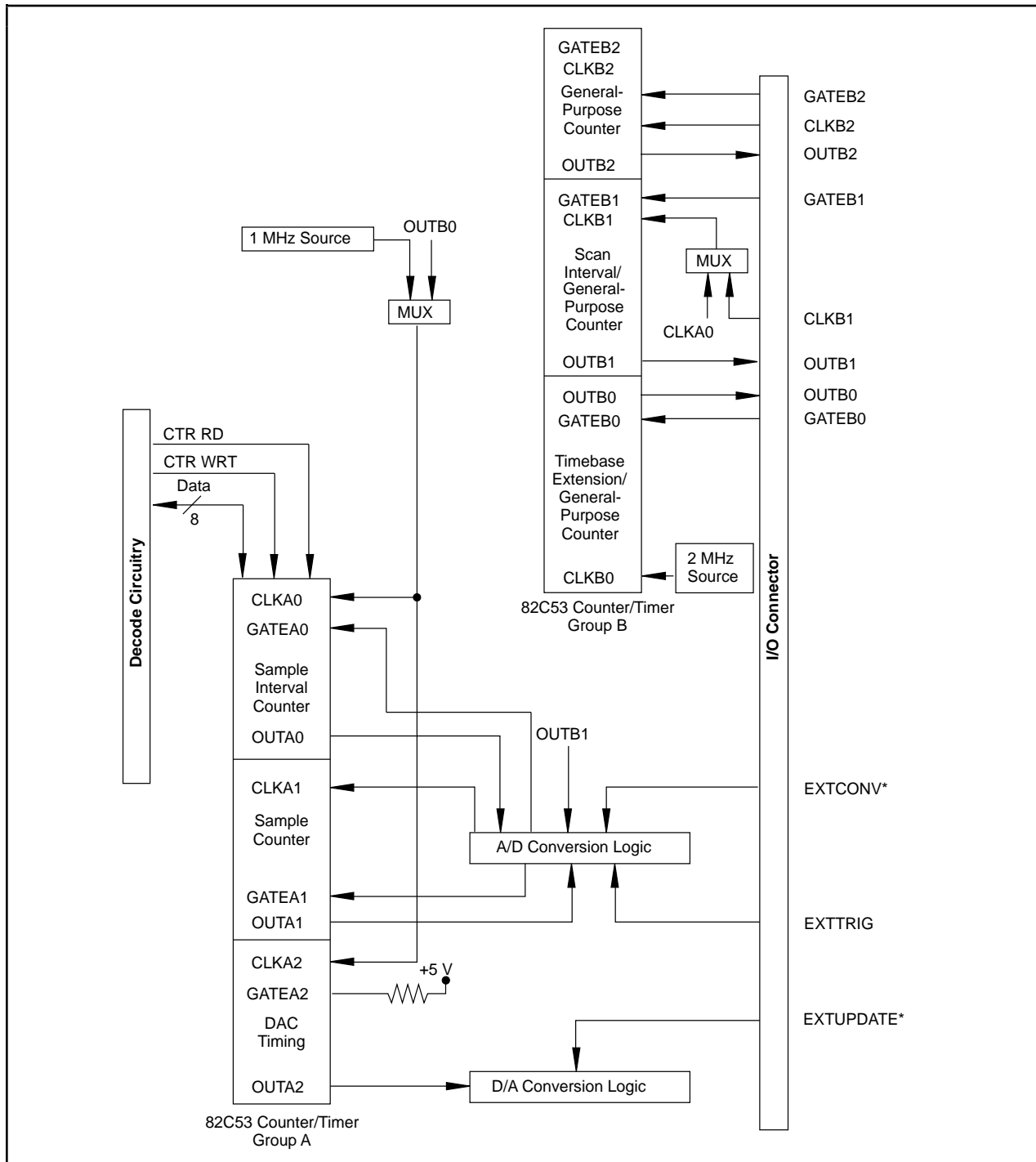
Figure 4-3. Timing Circuitry
